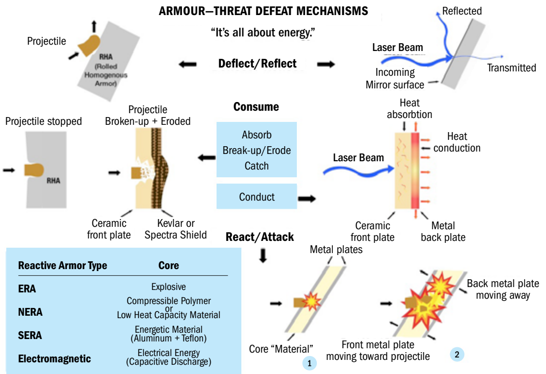
Figure 1. Summary of basic mechanisms for defeating an incoming projectile or laser beam.
