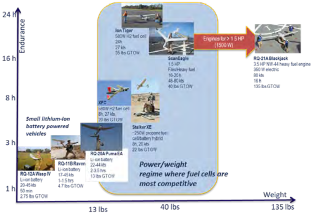
Figure 3. Tier 1 to tier 3 battery, fuel cell, and engine-powered UAS: comparison of propulsion/energy source, speed, endurance and gross takeoff weight (GTOW).
