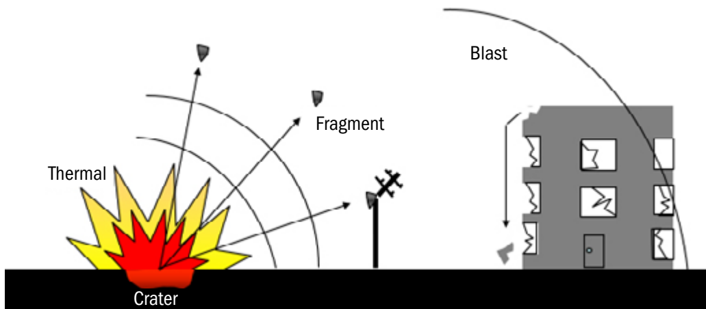
Figure 2. Graphical depiction of the basic effects of an explosion, with near-, mid- and far-field damage occurring from direct-pressure effects, thermal radiation within the fireball, fragmentation, and blast-wave damage.
