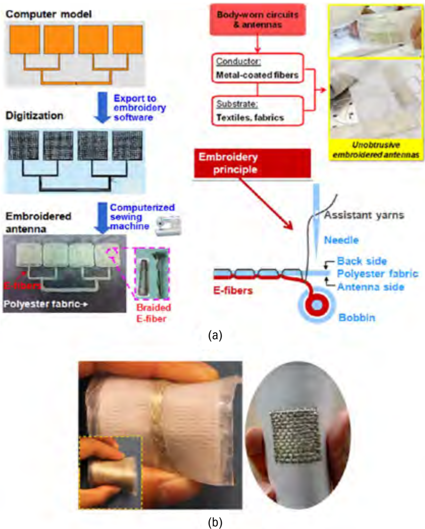
Figure 2. (a) Fabrication process of body-worn antennas, sensors, and RF circuits. These E-fiber RF components offer several new functionalities unavailable previously, such as inconspicuous weaving into garments, omnidirectional high-strength signals for connecting faraway cell towers and even satellites, and excellent conformality for interior body imaging. (b) Fabricated textile transmission line and patch antenna after placement onto a polymer substrate. 28
